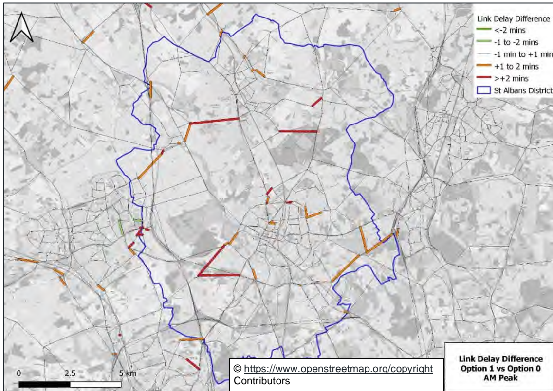
Figure 9-14: Link Delay Difference Option 1 vs Option 0 AM Peak
