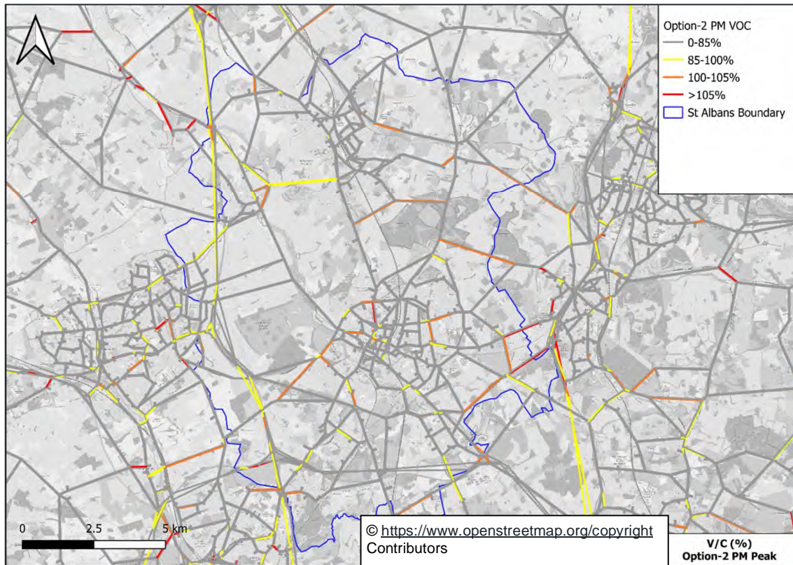
Figure 9-9: Option 2 Link Volume/Capacity Ratio, PM Peak Hour
