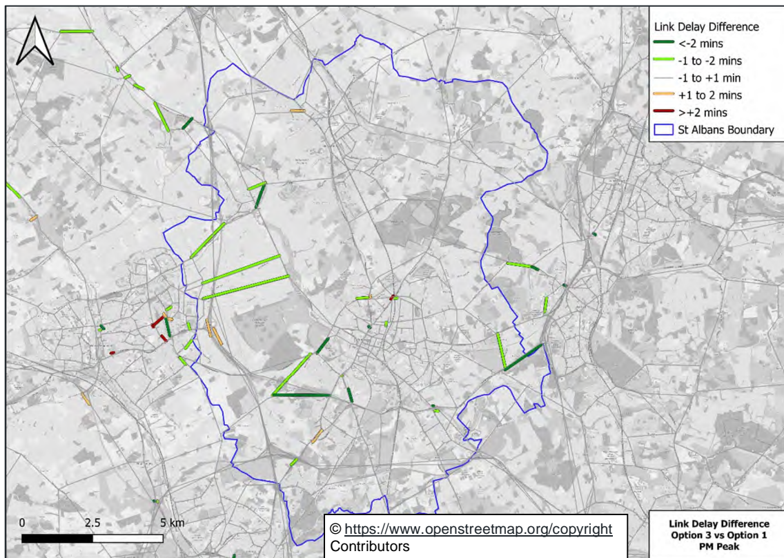
Figure 9-19: Link Delay Difference Option 3 vs Option 1 PM Peak
