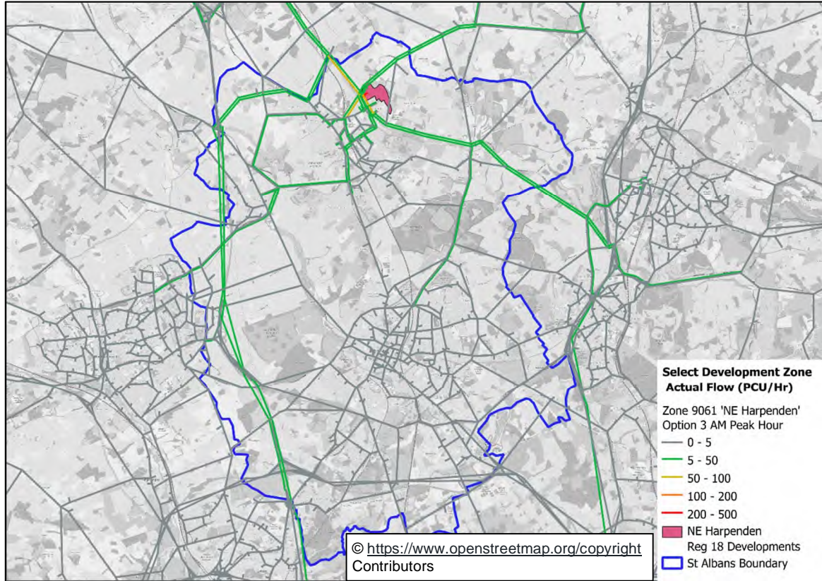
Figure 9-34: Traffic to and from North East Harpenden Development (AM Peak) Option 3
