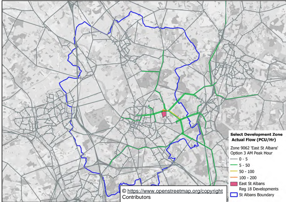
Figure 9-38: Traffic to and from East St Albans Development (AM Peak) Option 3
