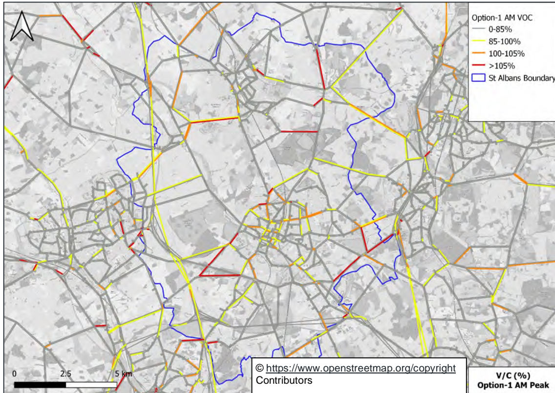
Figure 9-6: Option 1 Link Volume/Capacity Ratio, AM Peak Hour
