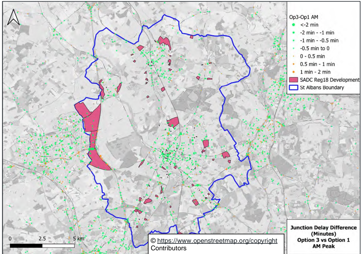
Figure 9-78: Node Delay Difference Option 3 vs Option 1 AM Peak
