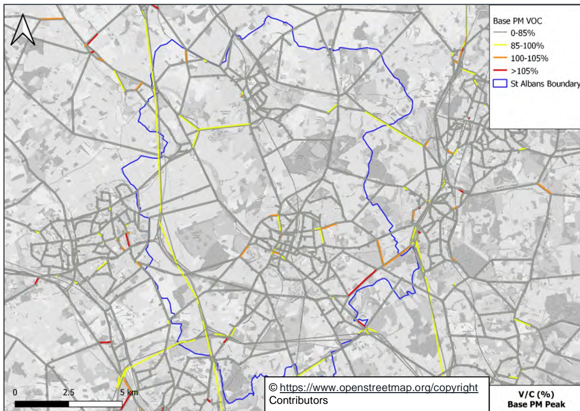
Figure 9-3: Base Year Link Volume/Capacity Ratio PM Peak Hour
