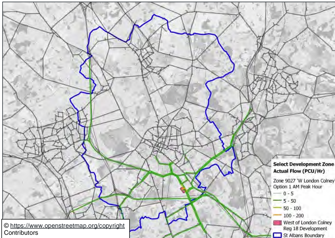
Figure 9-28: Traffic to and from West of London Colney Development (AM Peak) Option 1
