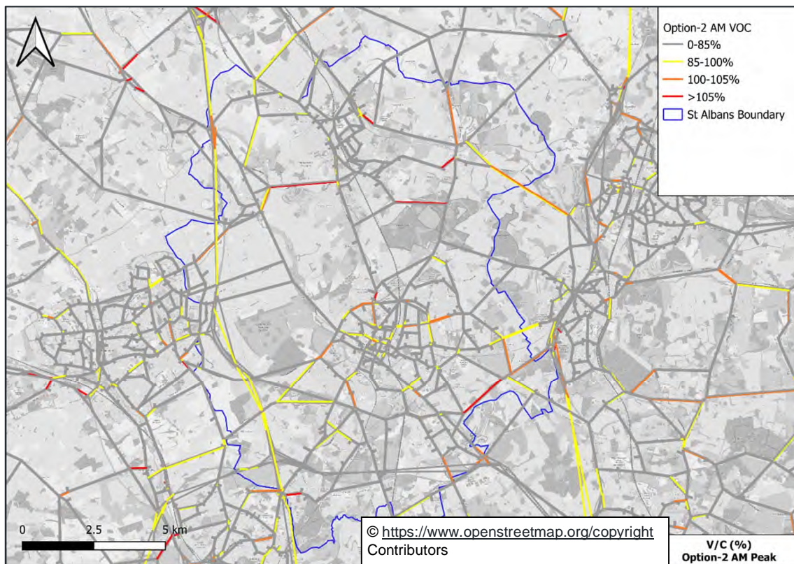
Figure 9-8: Option 2 Link Volume/Capacity Ratio, AM Peak Hour
