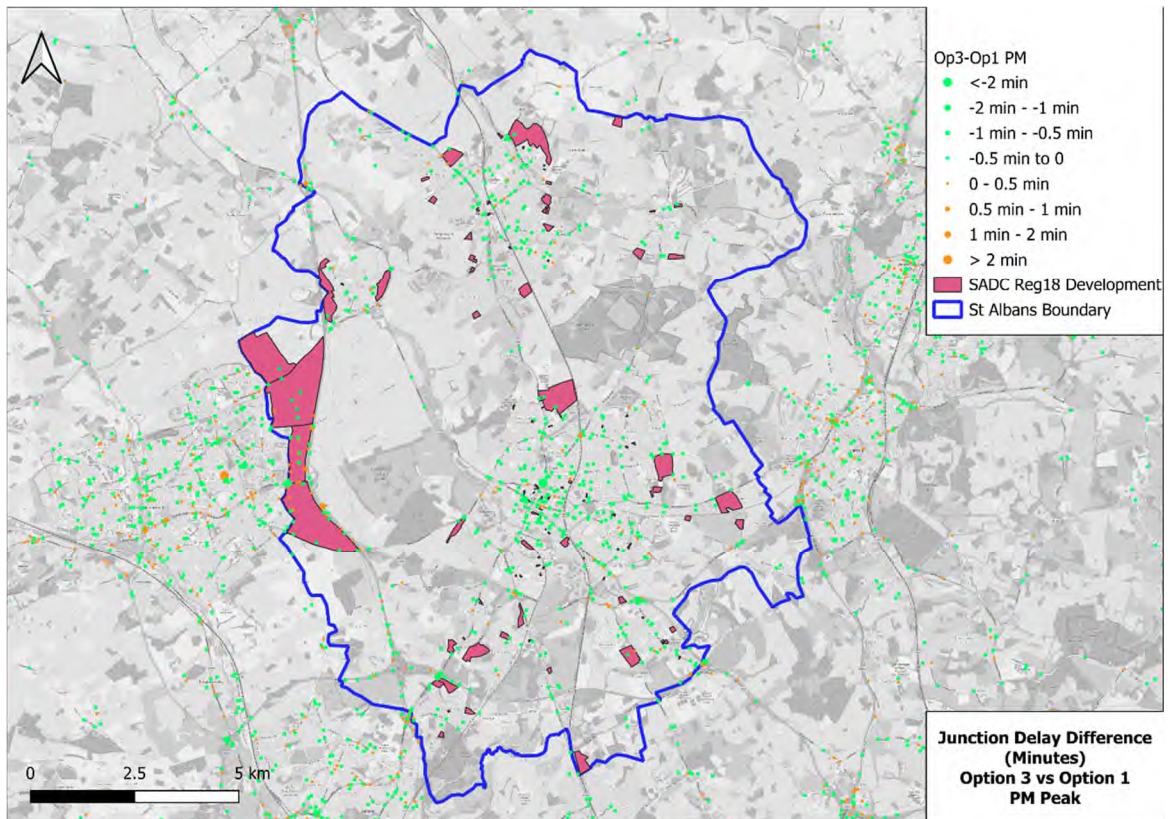
Figure 9-79: Node Delay Difference Option 3 vs Option 1 PM Peak
