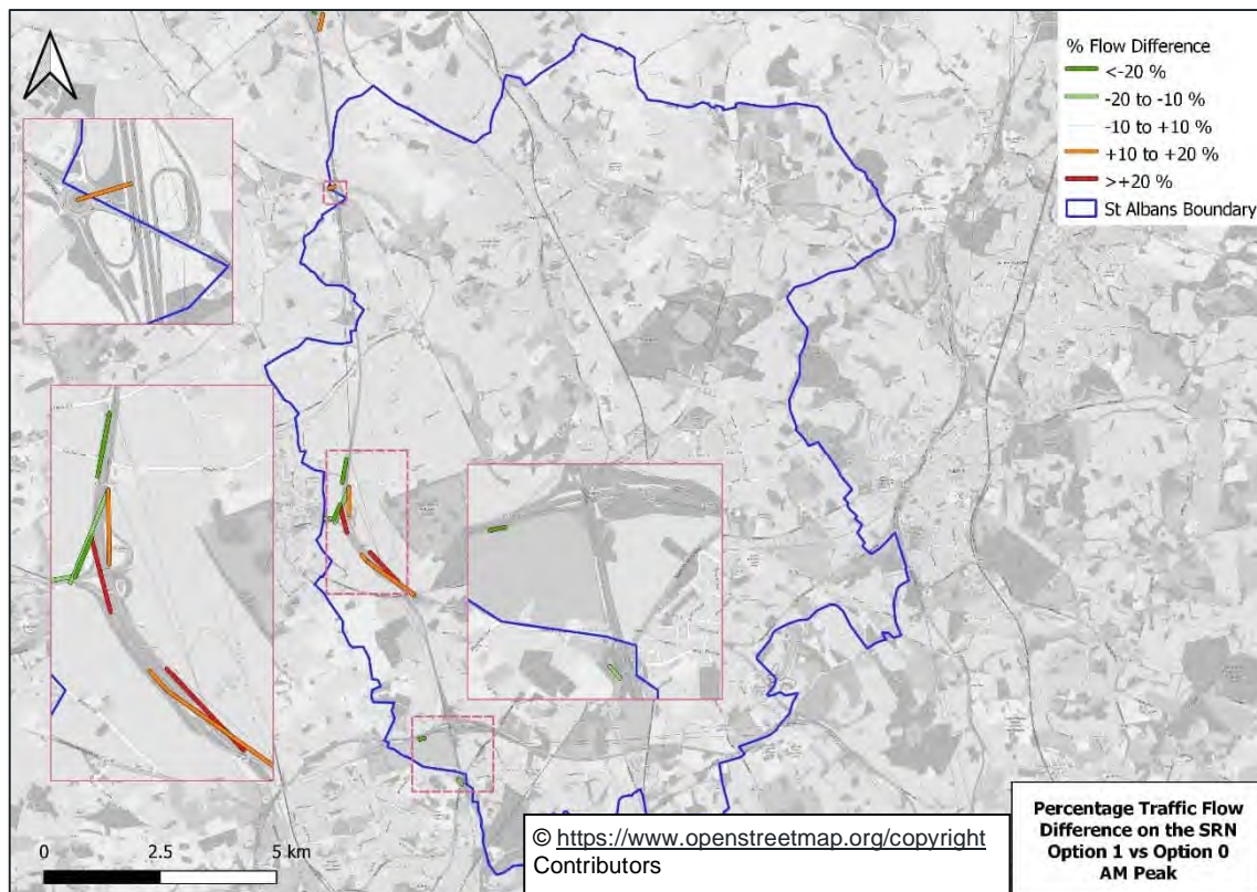
Figure 9-66: % Changes in Traffic Flow on SRN between Option 1 and Option 0 (AM Peak)
