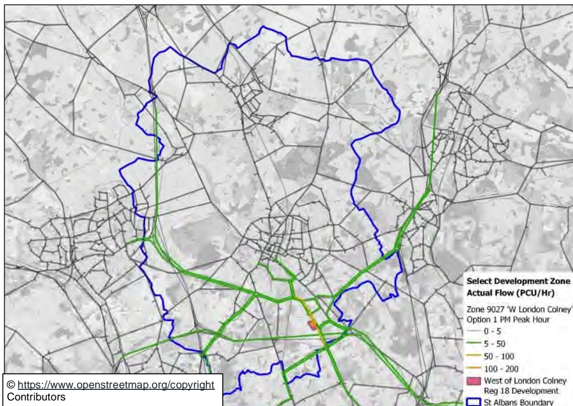
Figure 9-29: Traffic to and from West of London Colney Development (PM Peak) Option 1
