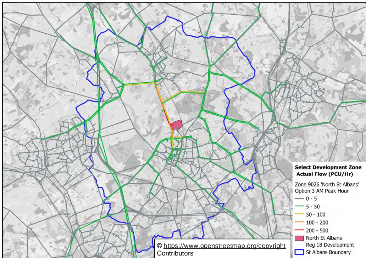
Figure 9-26: Traffic to and from North St Albans Development (AM Peak) Option 3
