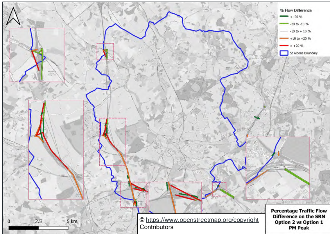
Figure 9-69: % Changes in Traffic Flow on SRN between Option 2 and Option 1 (PM Peak)
