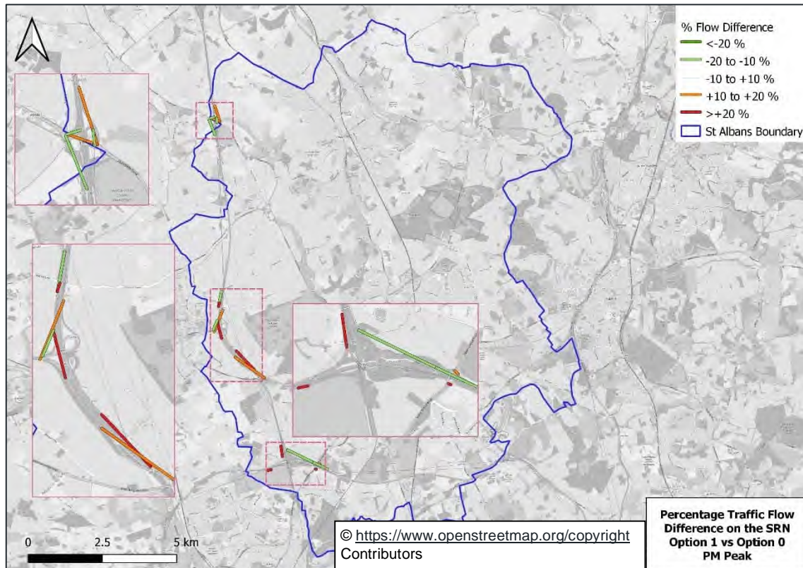
Figure 9-67: % Changes in Traffic Flow on SRN between Option 1 and Option 0 (PM Peak)
