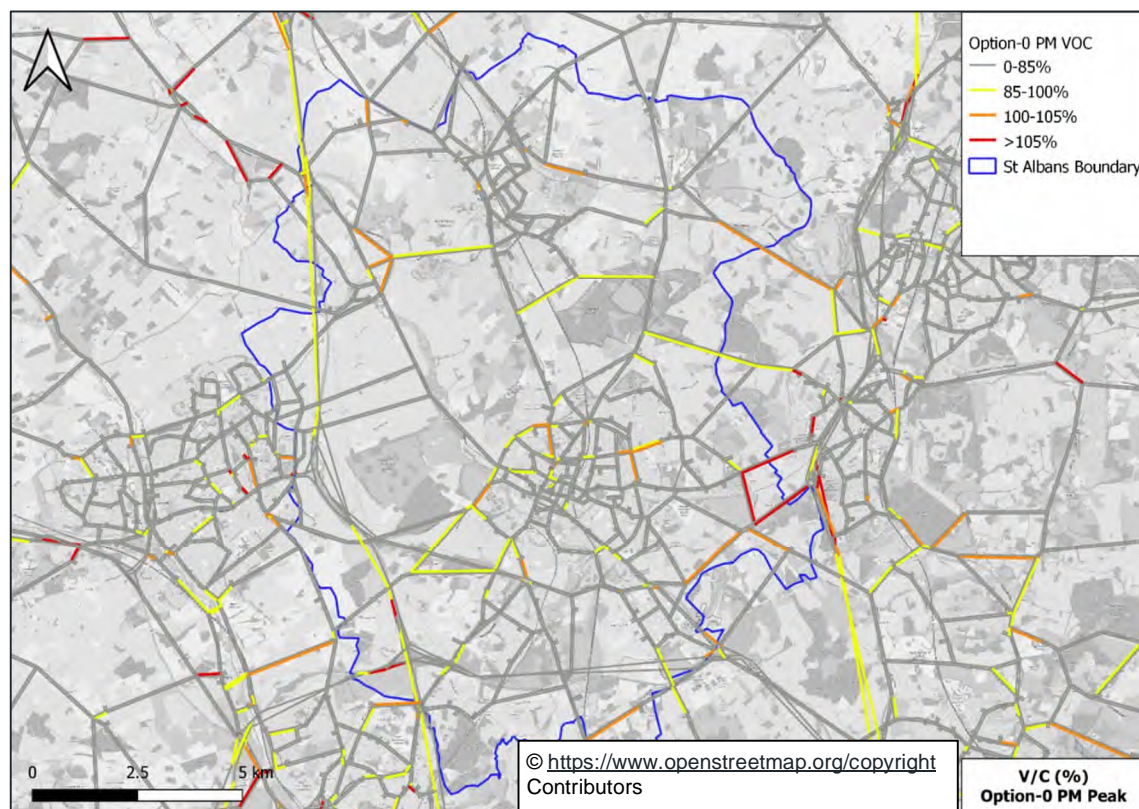
Figure 9-5: Option 0 Link Volume/Capacity Ratio, PM Peak Hour
