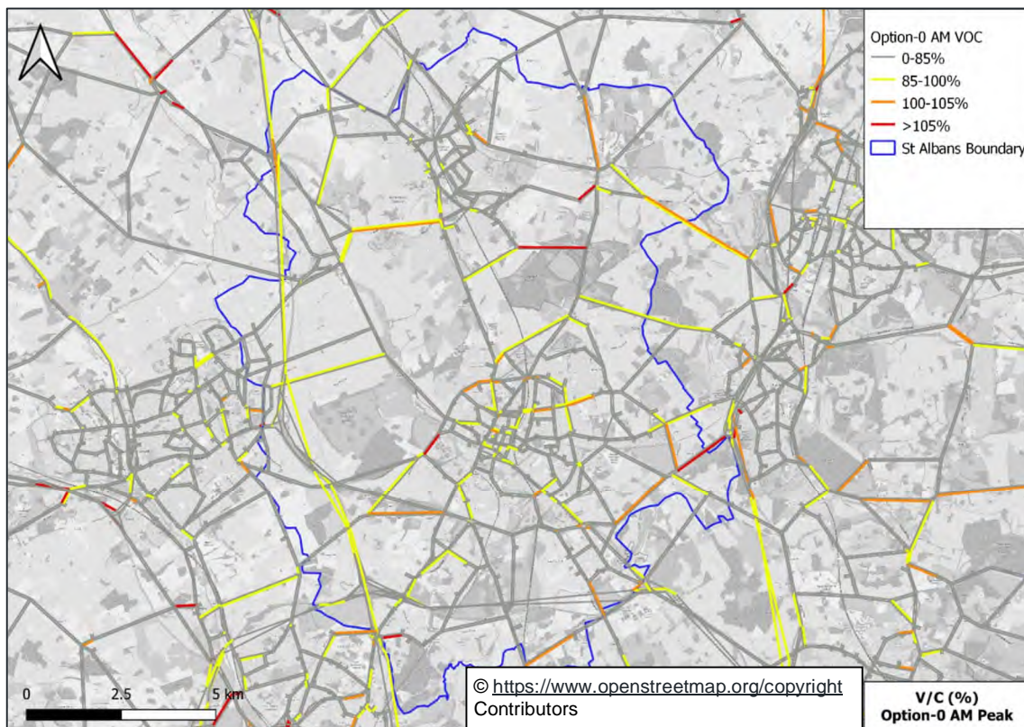
Figure 9-4: Option 0 Link Volume/Capacity Ratio, AM Peak Hour
