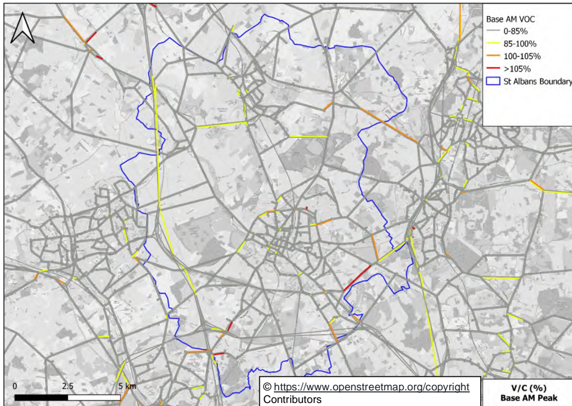
Figure 9-2: Base Year Link Volume/Capacity Ratio, AM Peak Hour
