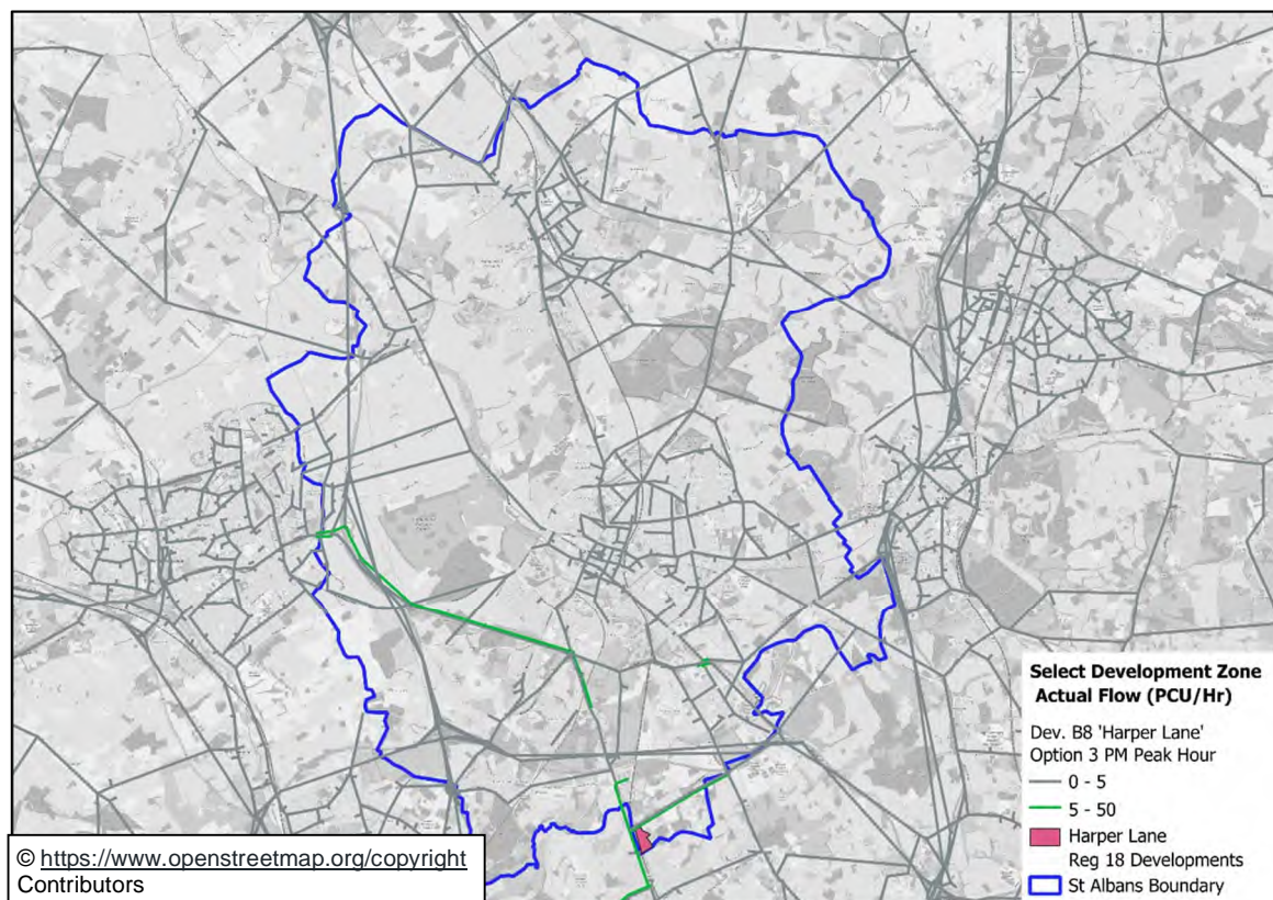
Figure 9-51: Traffic to and from Harper Lane Development (PM Peak) Option 3
