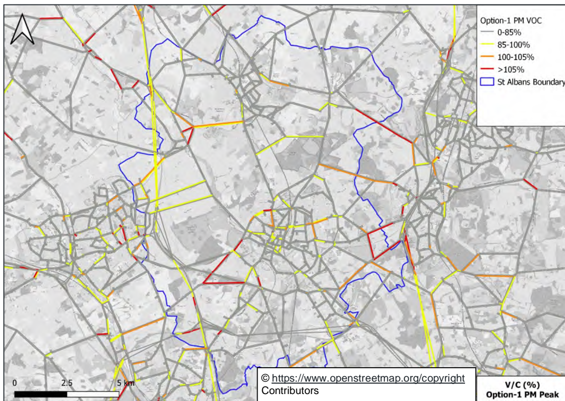
Figure 9-7: Option 1 Link Volume/Capacity Ratio, PM Peak Hour
