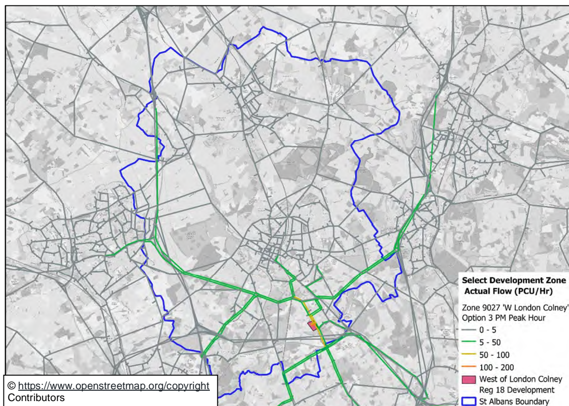
Figure 9-31: Traffic to and from West of London Colney Development (PM Peak) Option 3
