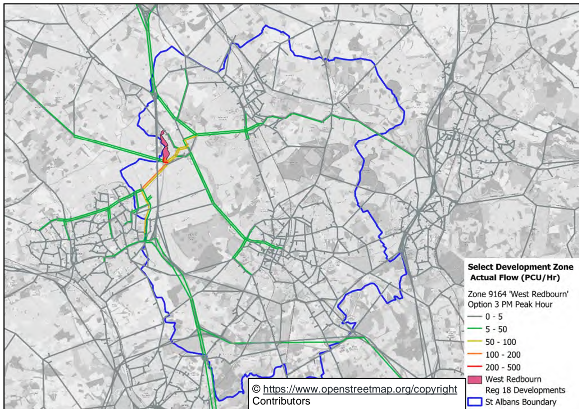
Figure 9-47: Traffic to and from West Redbourn Development (PM Peak) Option 3
