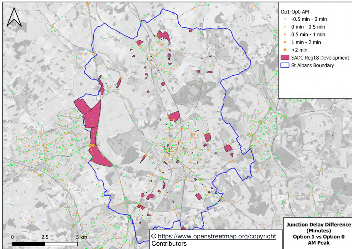
Figure 9-74: Node Delay Difference Option 1 vs Option 0 AM Peak
