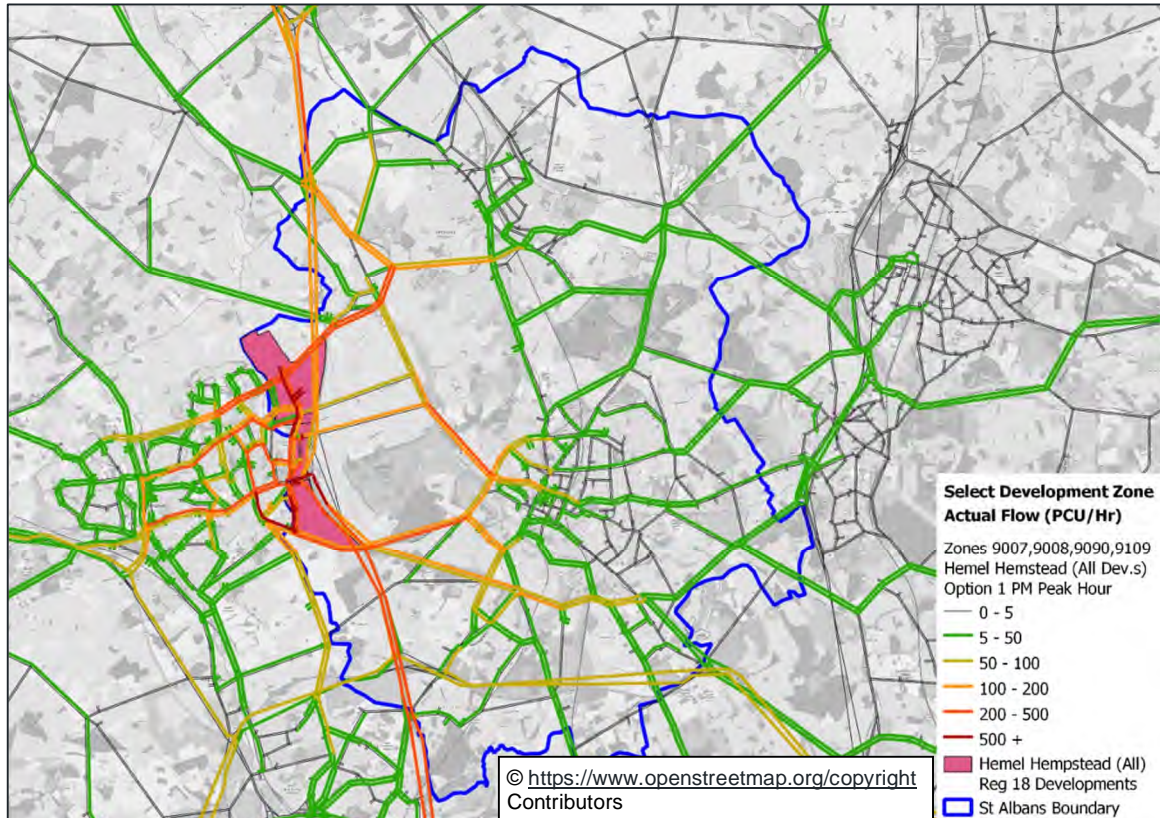
Figure 9-21: Traffic to and from East Hemel development (PM Peak) Option 1
