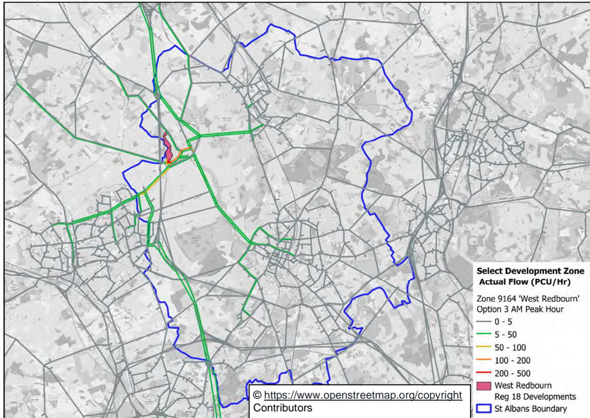
Figure 9-46: Traffic to and from West Redbourn Development (AM Peak) Option 3
