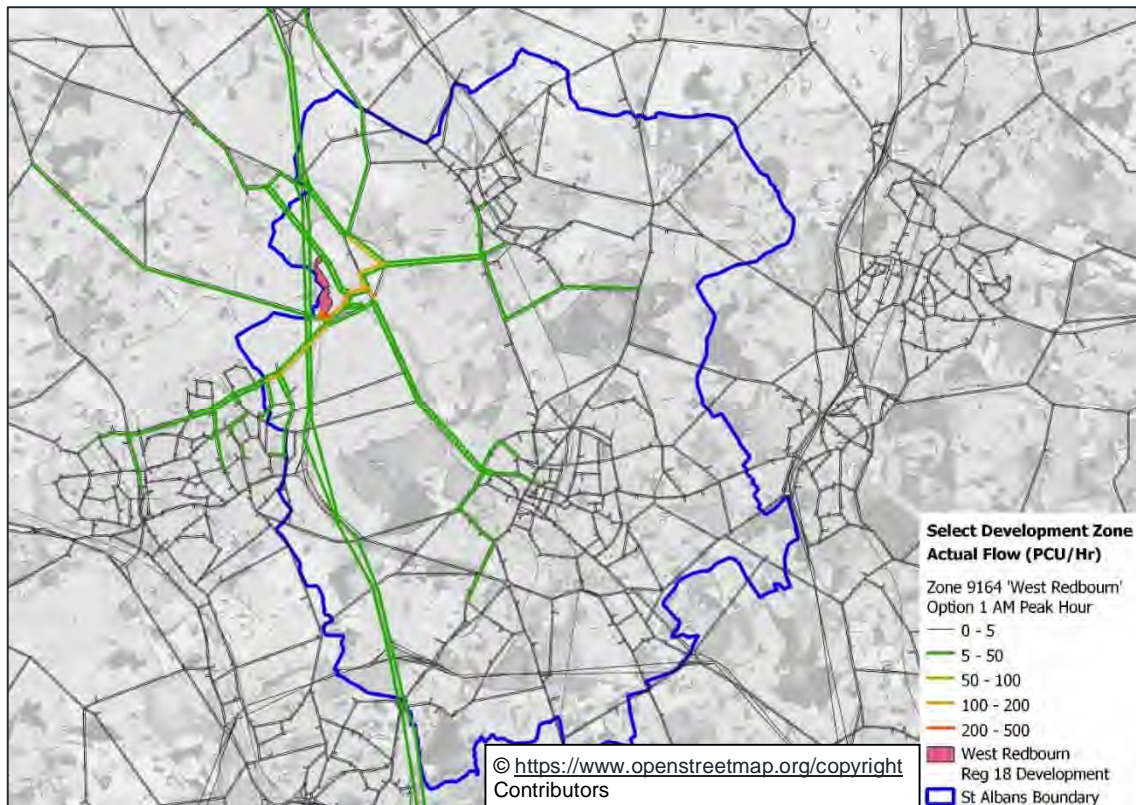
Figure 9-44: Traffic to and from West Redbourn Development (AM Peak) Option 1
