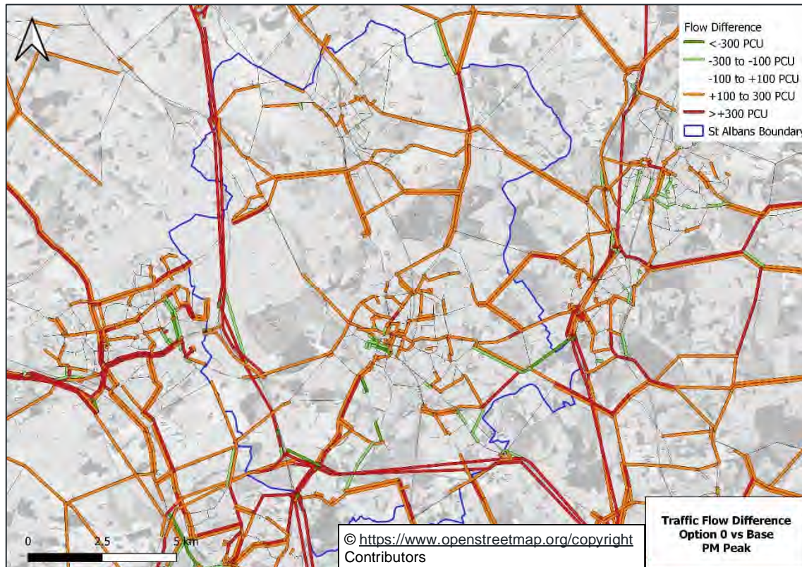
Figure 9-57: SAD Changes in Traffic Flow between Option 0 and Base Year (PM Peak)
