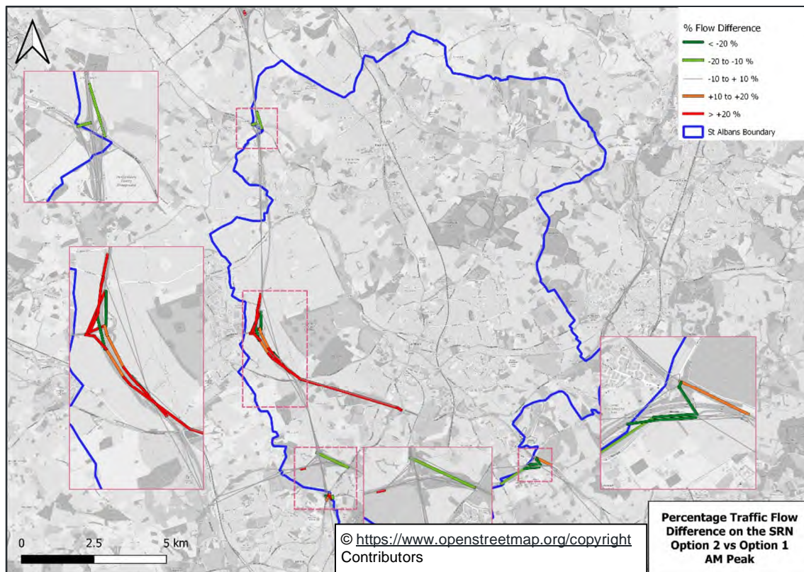
Figure 9-68: % Changes in Traffic Flow on SRN between Option 2 and Option 1 (AM Peak)
