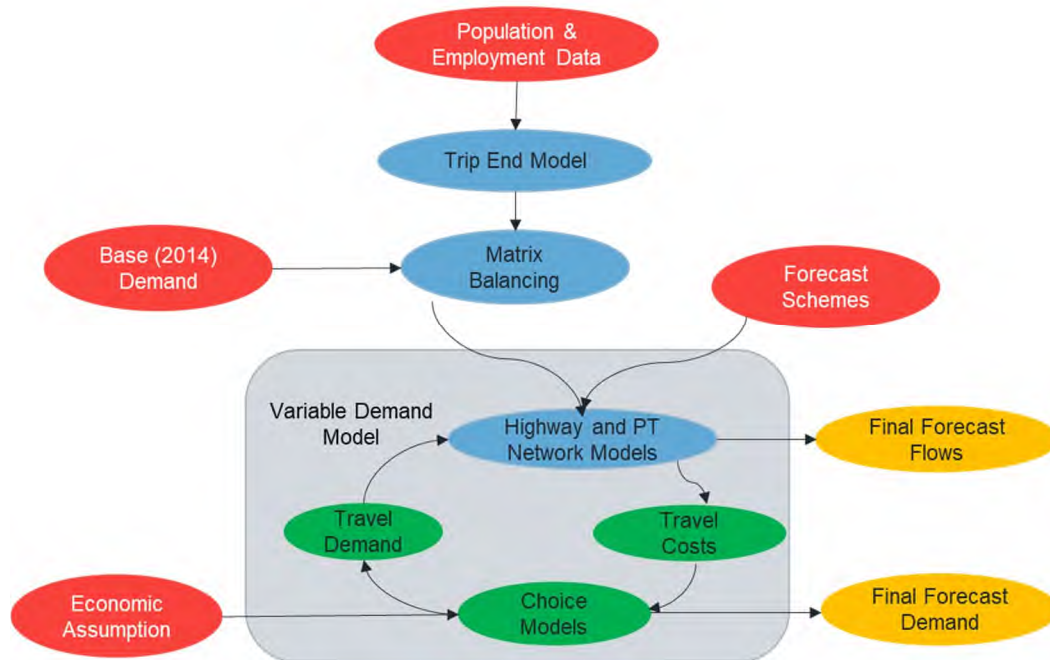
Figure 4-1: Model Structure
