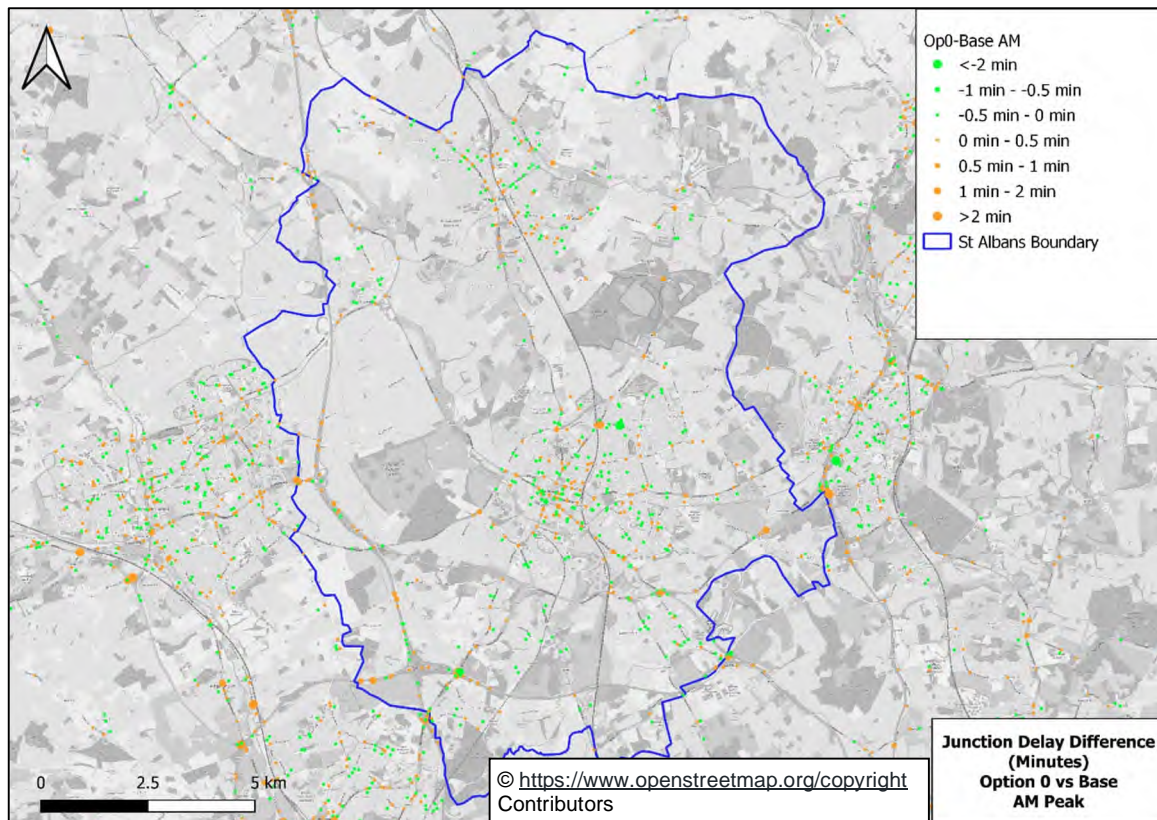
Figure 9-72: Node Delay Difference Option 0 vs Base AM Peak
