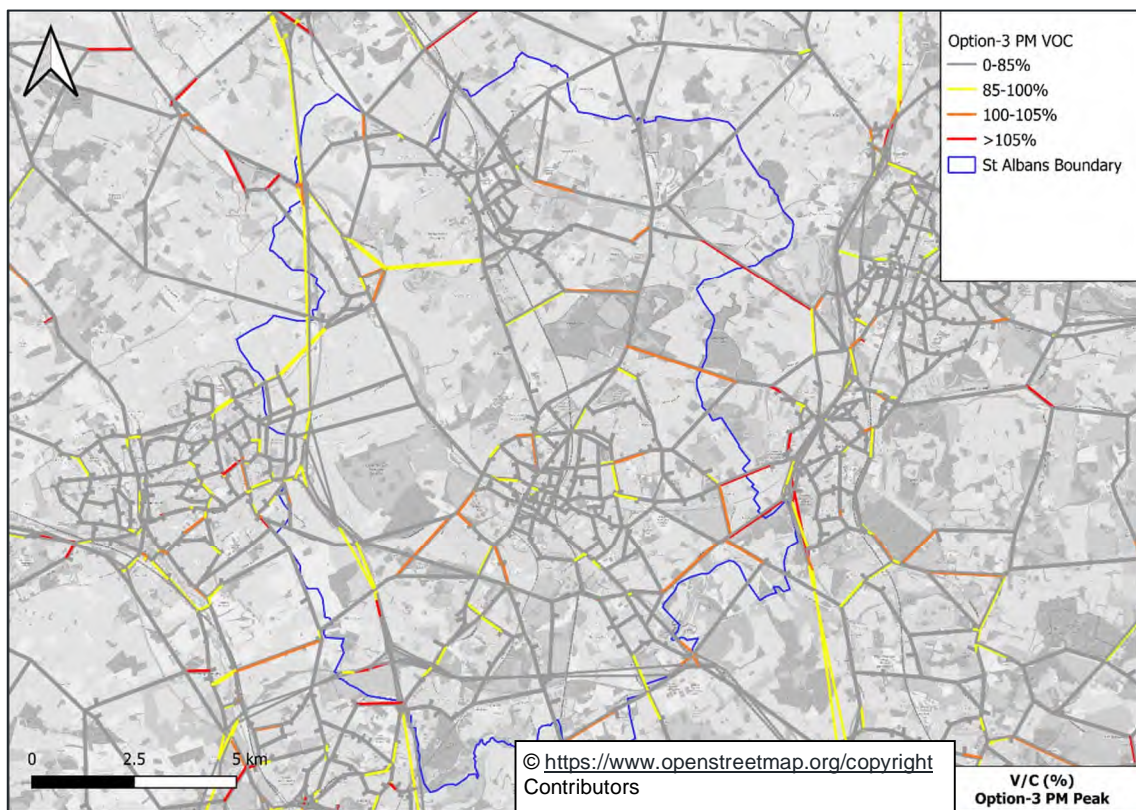
Figure 9-11: Option 3 Link Volume/Capacity Ratio, PM Peak Hour
