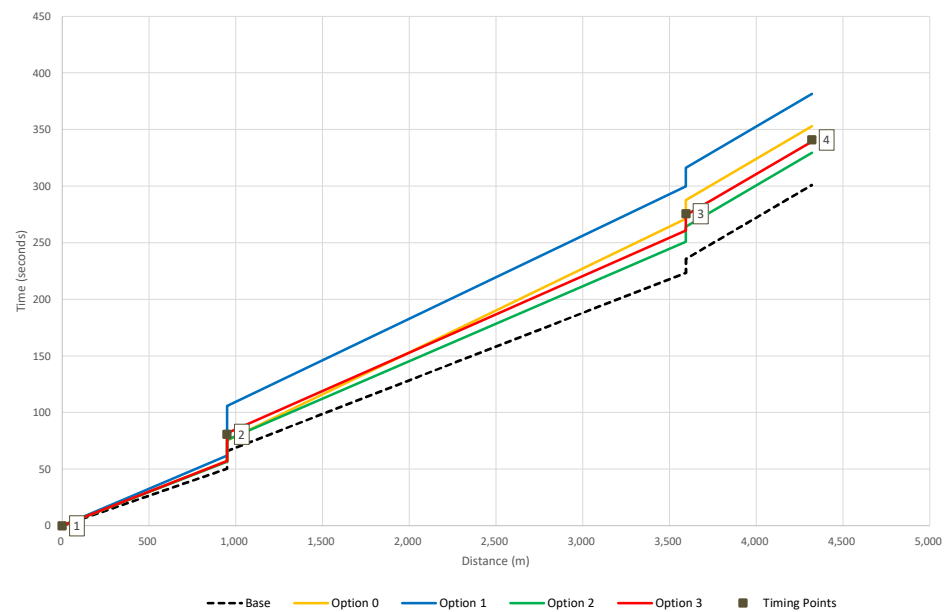
AM Peak Hour
