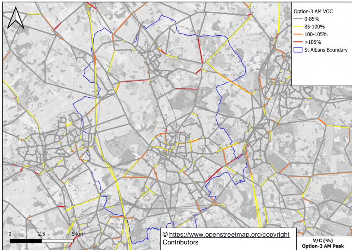
Figure 9-10: Option 3 Link Volume/Capacity Ratio, AM Peak Hour
