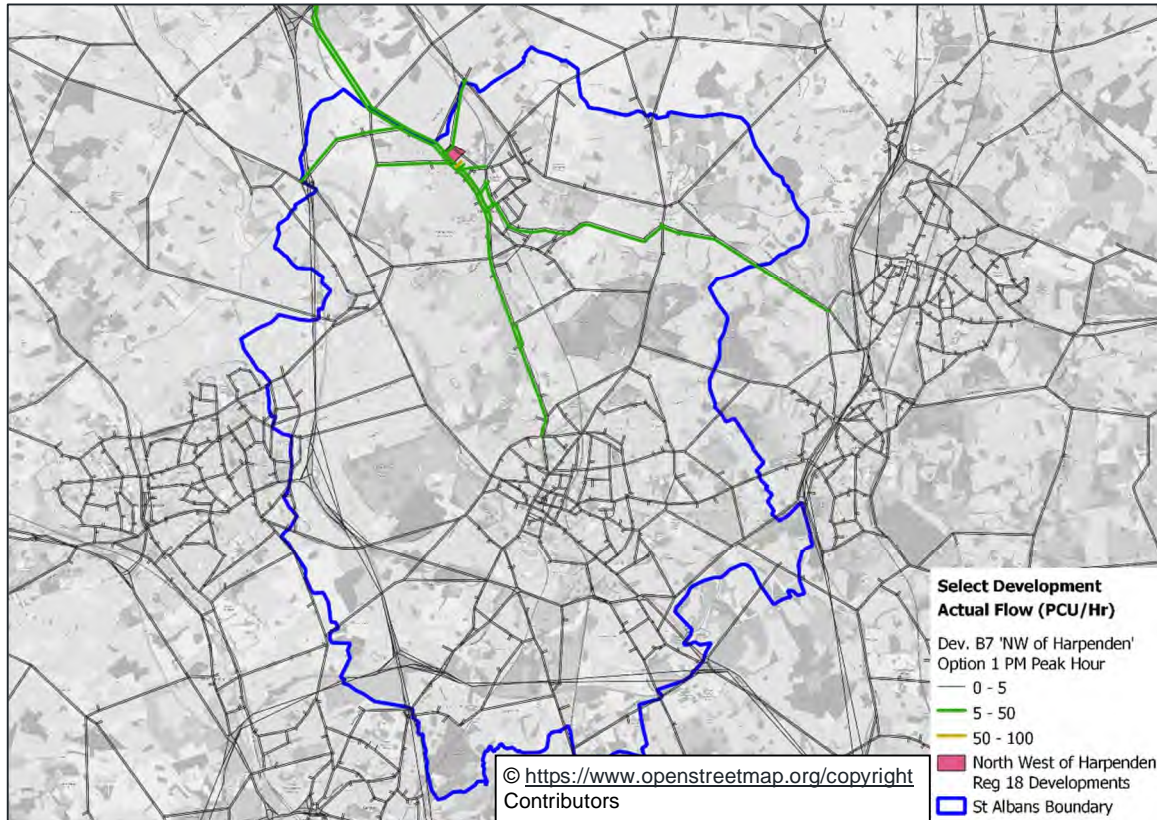
Figure 9-53: Traffic to and from North West Harpenden Development (PM Peak) Option 1
