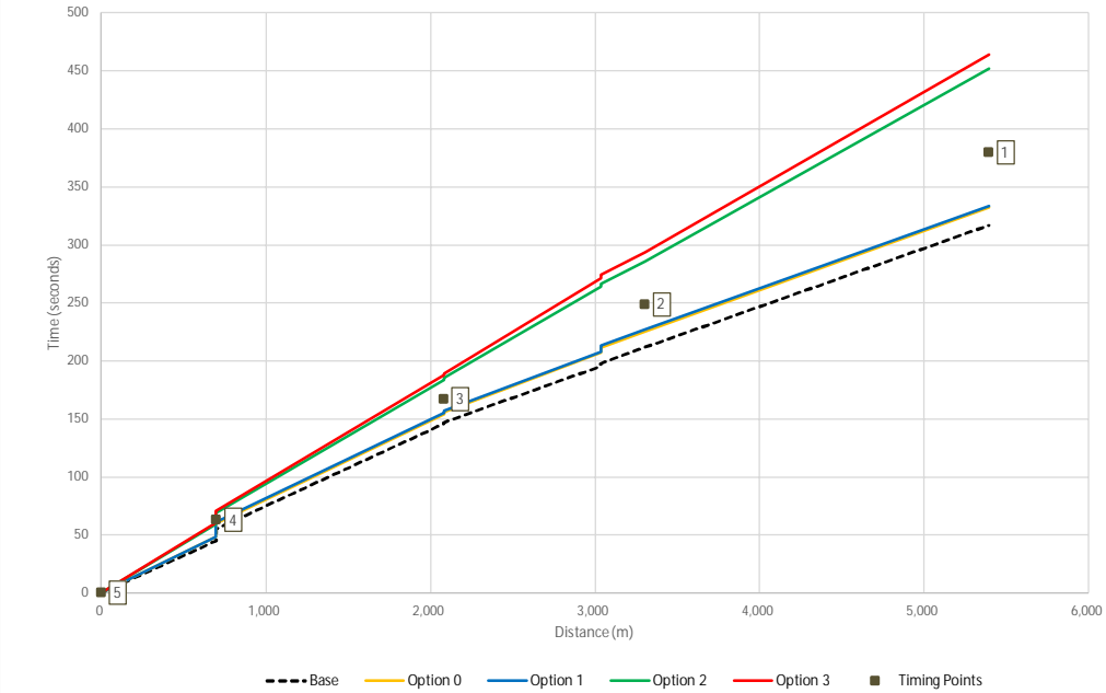
AM Peak Hour
