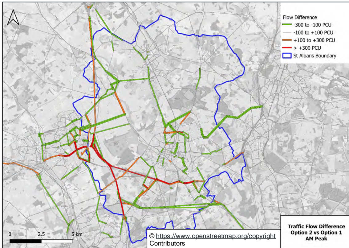
Figure 9-60: SAD Changes in Traffic Flow between Option 2 and Option 1 (AM Peak)
