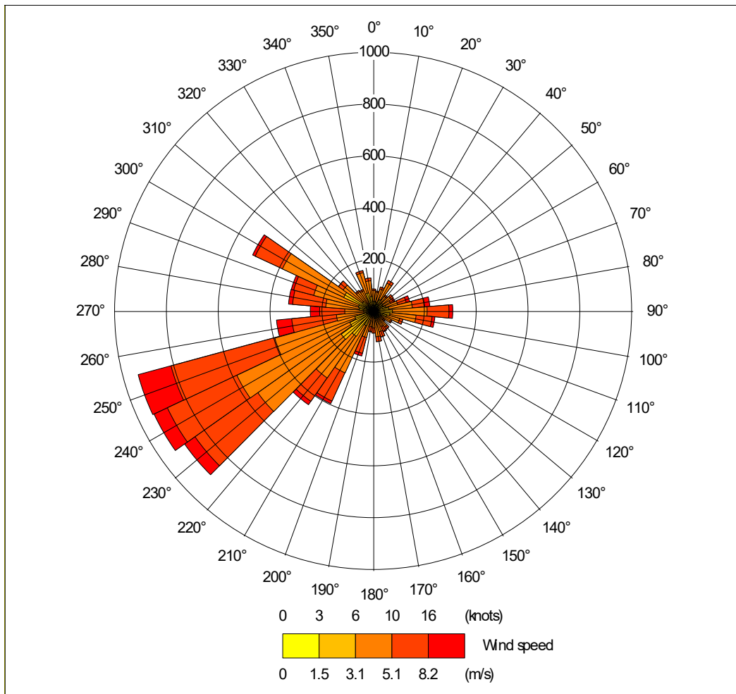
Wind Rose – London Luton Airport
