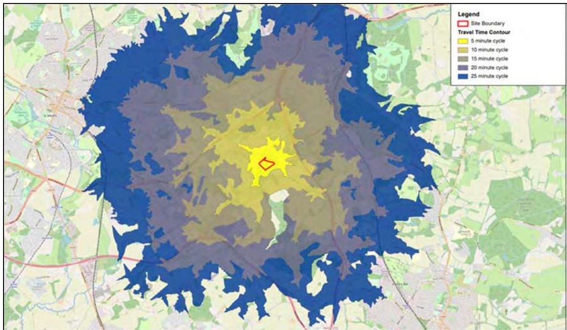
Figure 5: Cycle Isochrones
