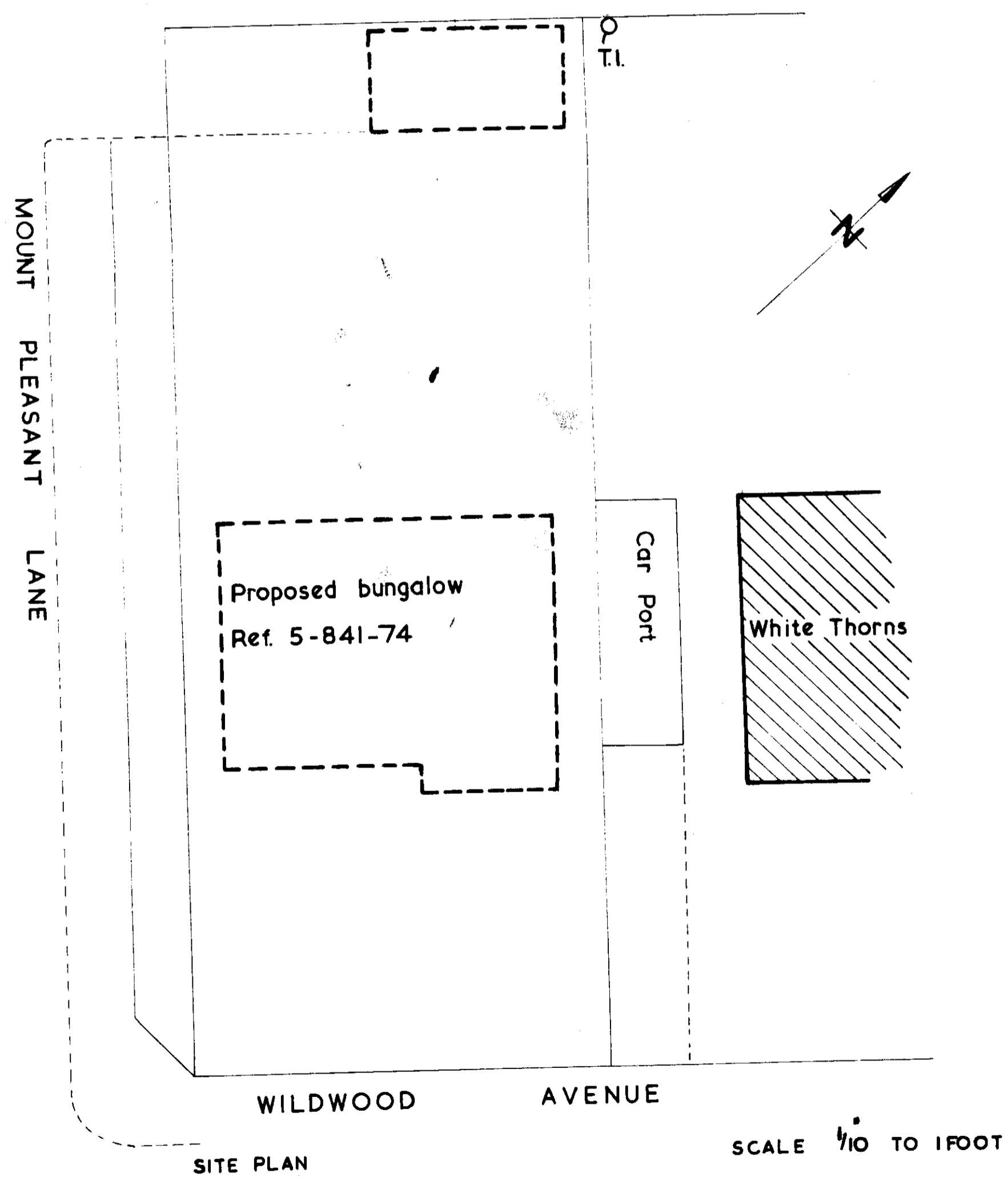
SITE PLAN
